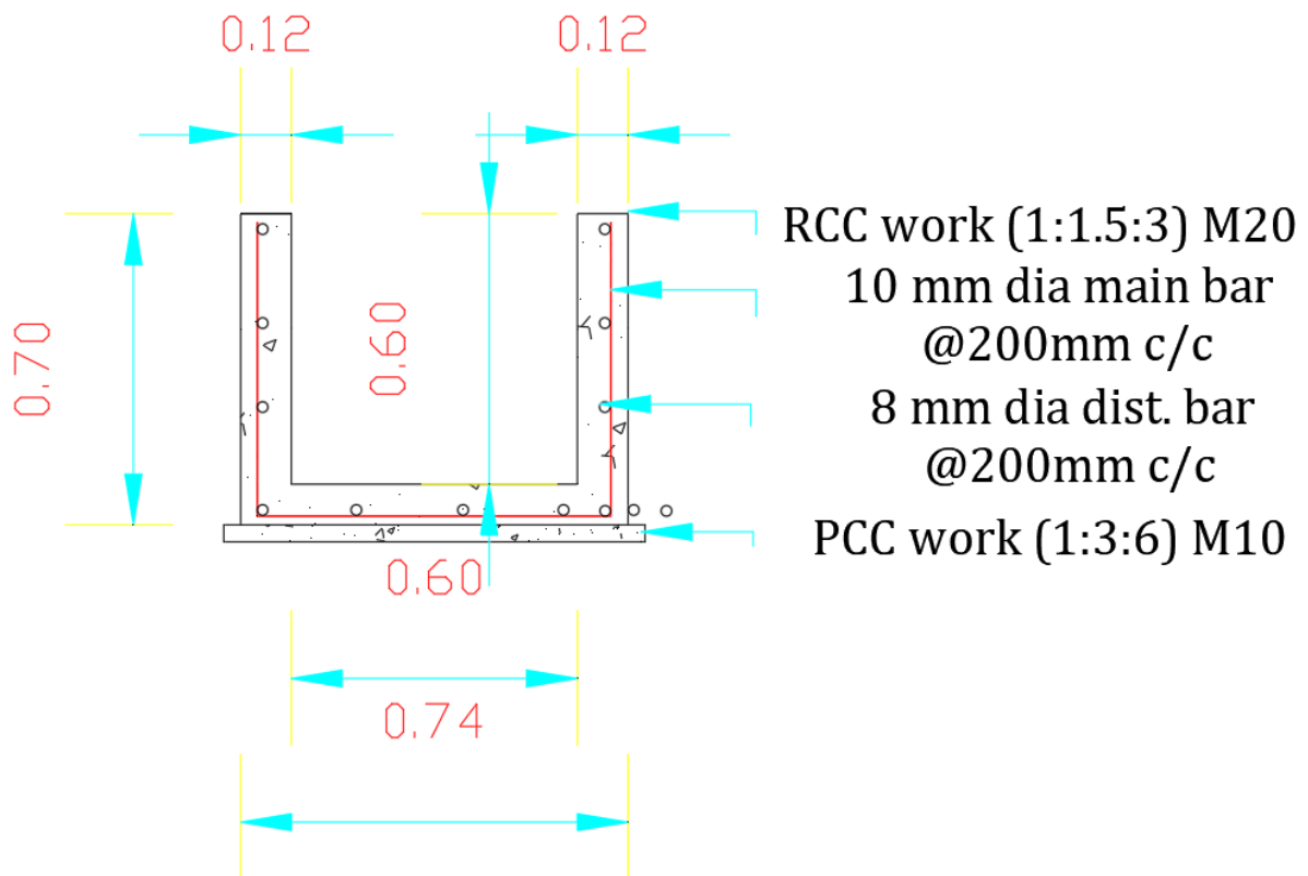
Fig: Canal Section at Ambasa IP
