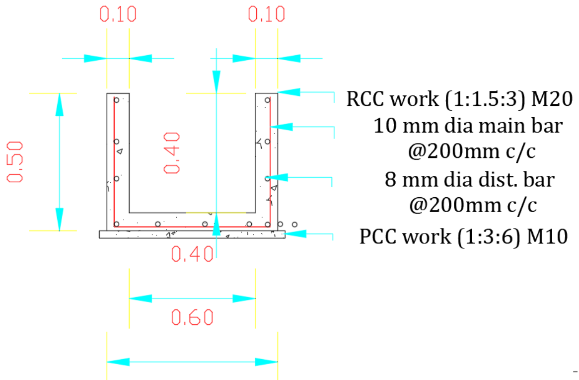
Fig: Canal Section at Karmala IP
